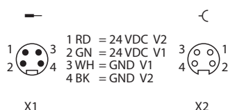
Fig. 20: TBEN-L4... – pin assignment of the power supply connections
