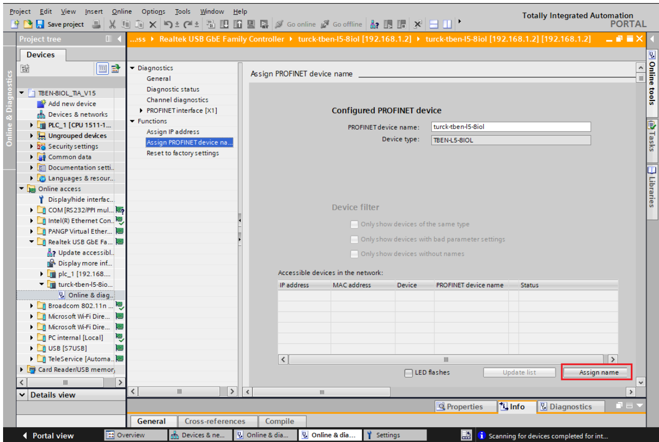
Fig. 38: TIA-Portal: Assigning the PROFINET device name
