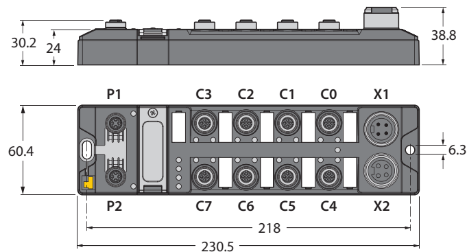
Fig. 1: Dimensions TBEN-L4-8IOL
