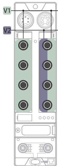
Fig. 22: Supply TBEN-L...-8IOL
