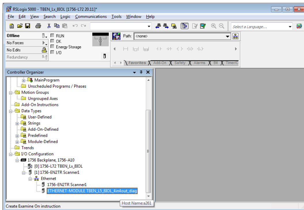
Fig. 65: Predefined configurations of TBEN-L...-8IOL in new project
