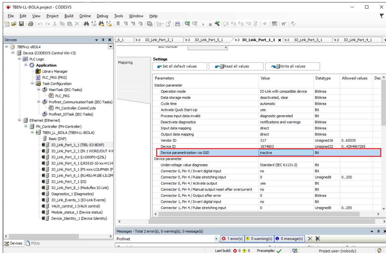
Fig. 92: PROFINET engineering (CODESYS); Device parameterization via GSD inactive
