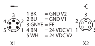
Fig. 21: TBEN-L5... – pin assignment of the power supply connections
