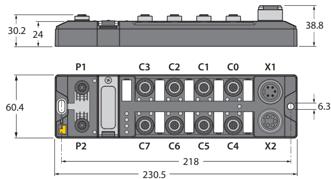
Fig. 2: Dimensions TBEN-L5-8IOL
