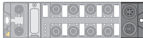
Fig. 19: TBEN-L5... – 7/8" connector for connecting the power supply
