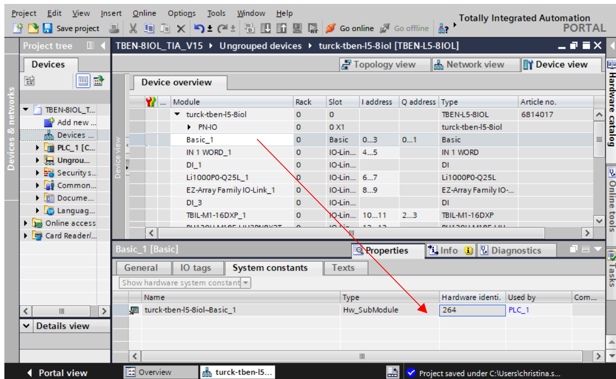
Fig. 44: Hardware identifier: Basic slot of the TBEN-L...-8IOL in the example
