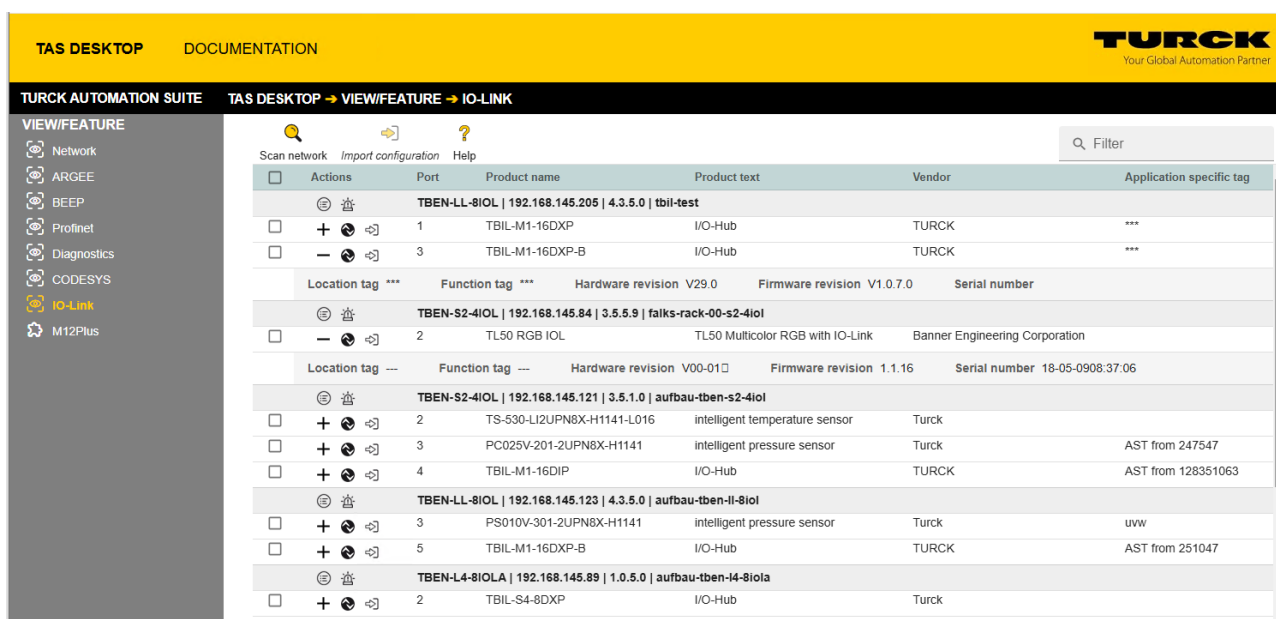
Fig. 95: TAS - IO-Link masters and devices found
