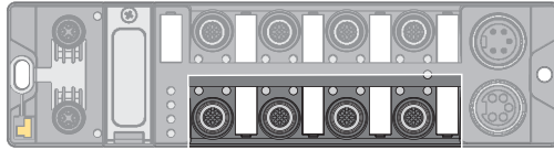
Fig. 25: M12 connectors, IO-Link master ports, Class B
