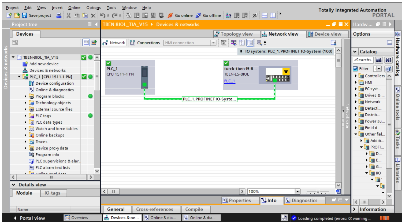
Fig. 42: TIA-Portal: Online mode
