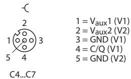
Fig. 26: Pin assignment of IO-Link master ports, Class B, C4...C7
