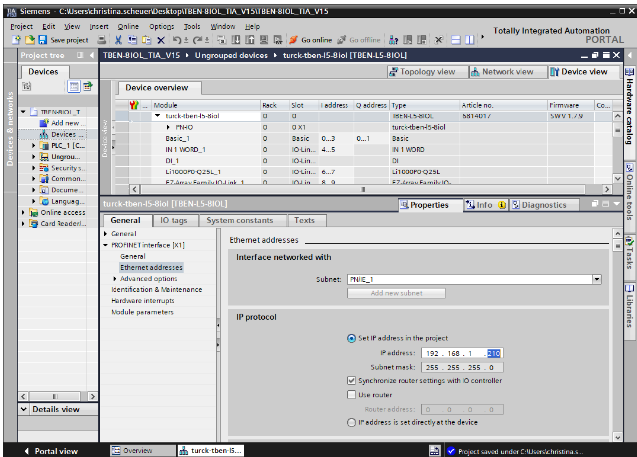
Fig. 39: TIA-Portal: Assigning the IP address
