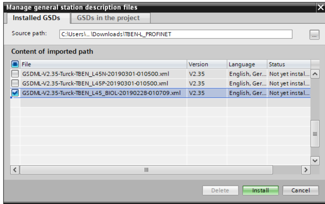
Fig. 36: TIA Portal: Installing the GSDML-file
