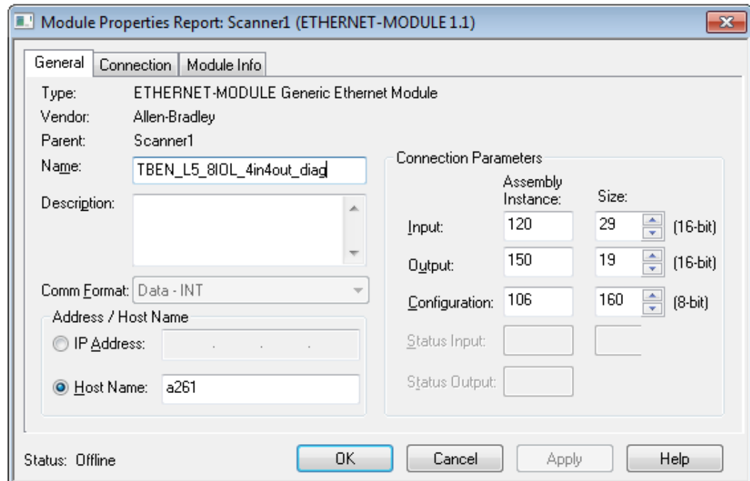
Fig. 66: Setting the module name and the IP address or respectively the host name
