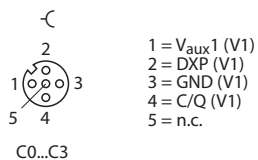
Fig. 24: Pin assignment of IO-Link master ports, Class A, C0...C3
