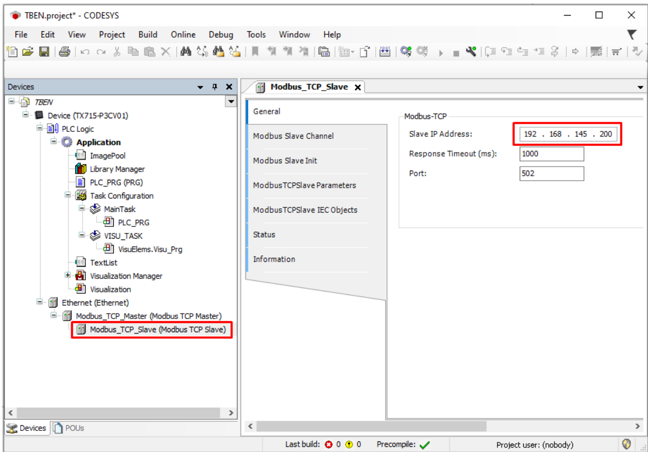
Fig. 57: Modbus TCP Slave: Setting the IP address
