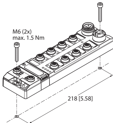
Fig. 10: Mounting the device onto a mounting plate
