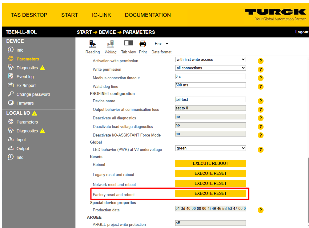
Fig. 99: TAS – resetting the device to factory settings
