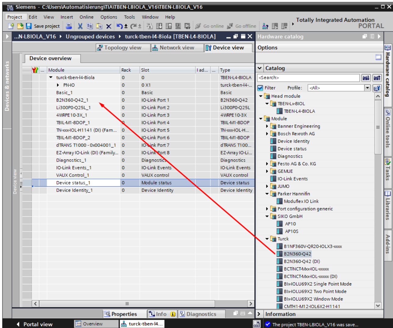
Fig. 89: Example: TIA Portal, IO-Link device in hardware catalog (SIDI)
