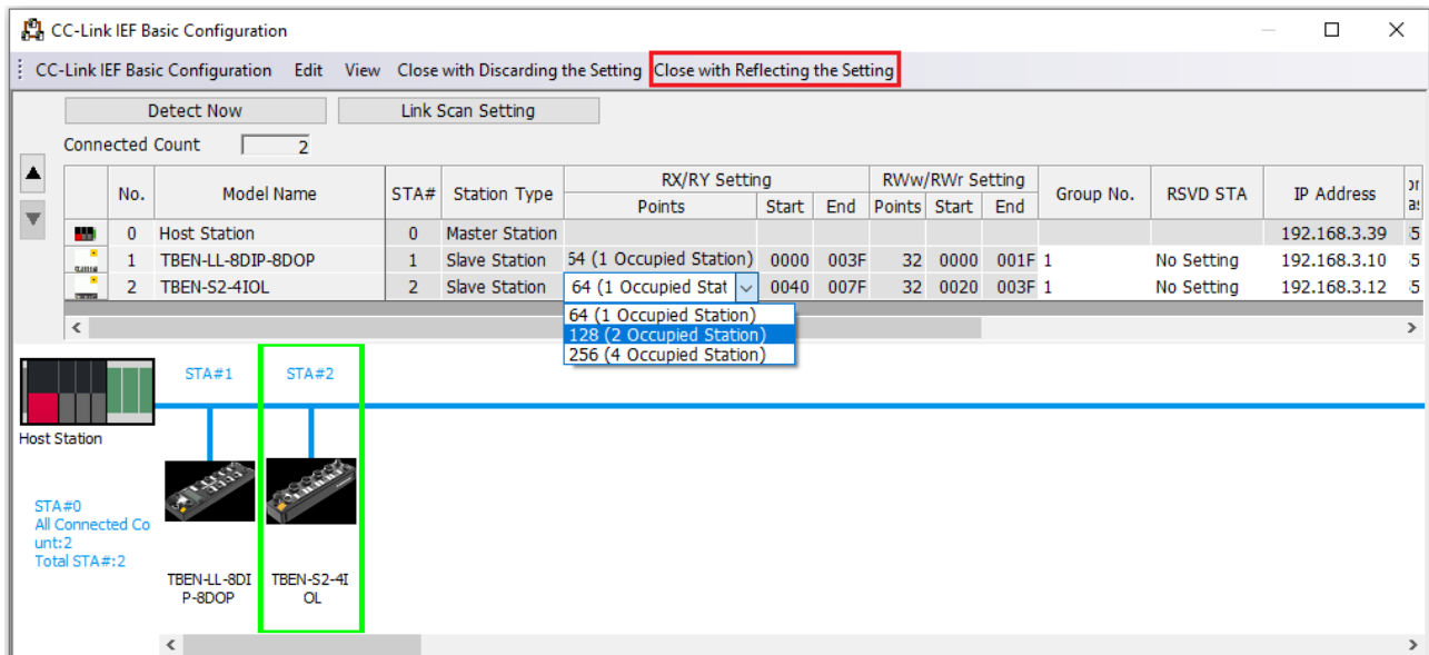
Fig. 79: GX Works3: Storing the network structure
