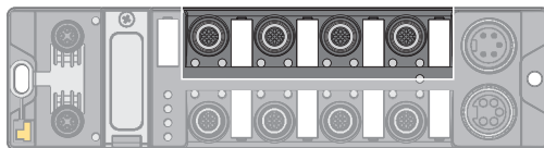
Fig. 23: M12 connectors, IO-Link master ports, Class A
