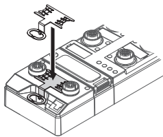
Fig. 15: Mounting the grounding clip
