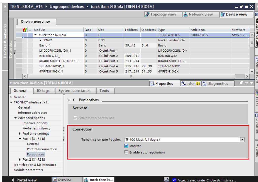
Fig. 34: TIA-Portal – port-settings for FSU
