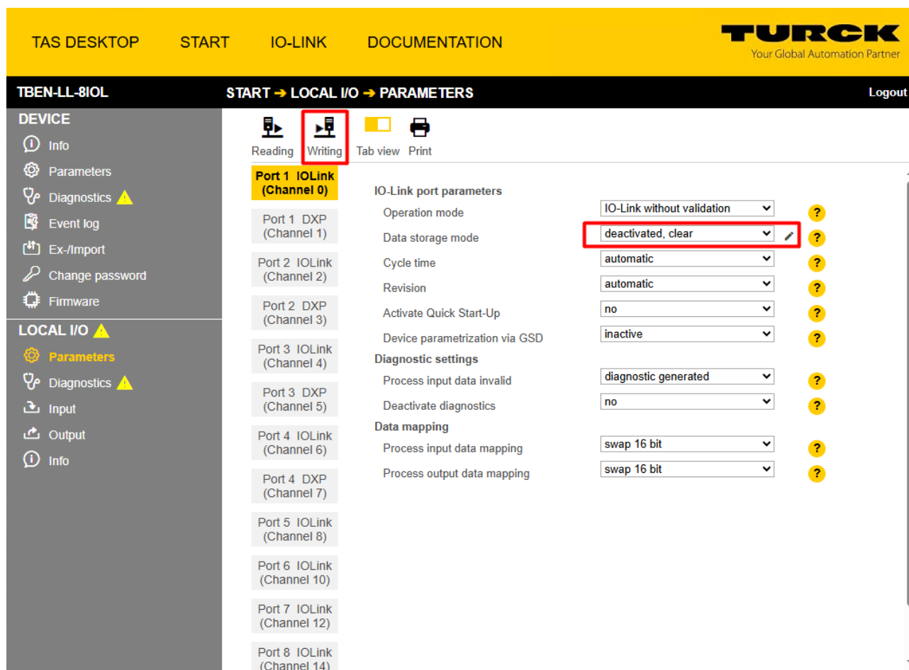
Fig. 98: TAS – deactivate data storage
