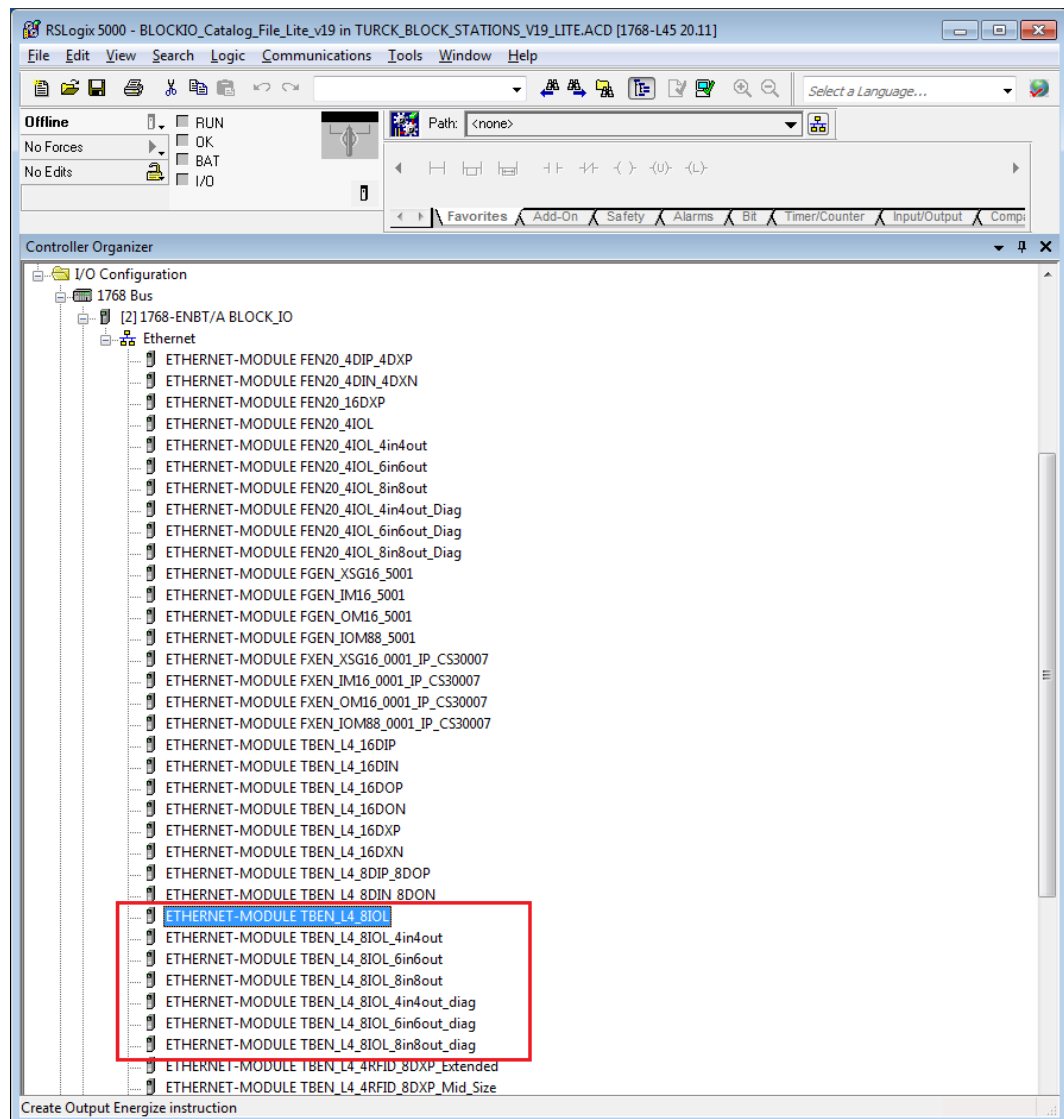
Fig. 64: Copying the device entry from catalog file
