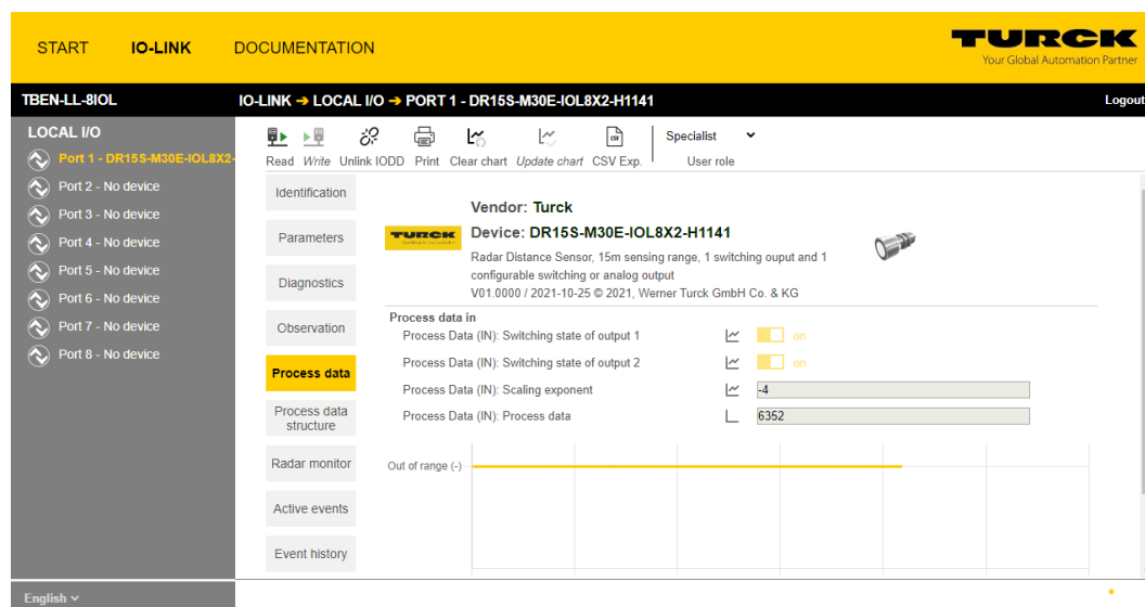
Fig. 109: Process data of an IO-Link device
