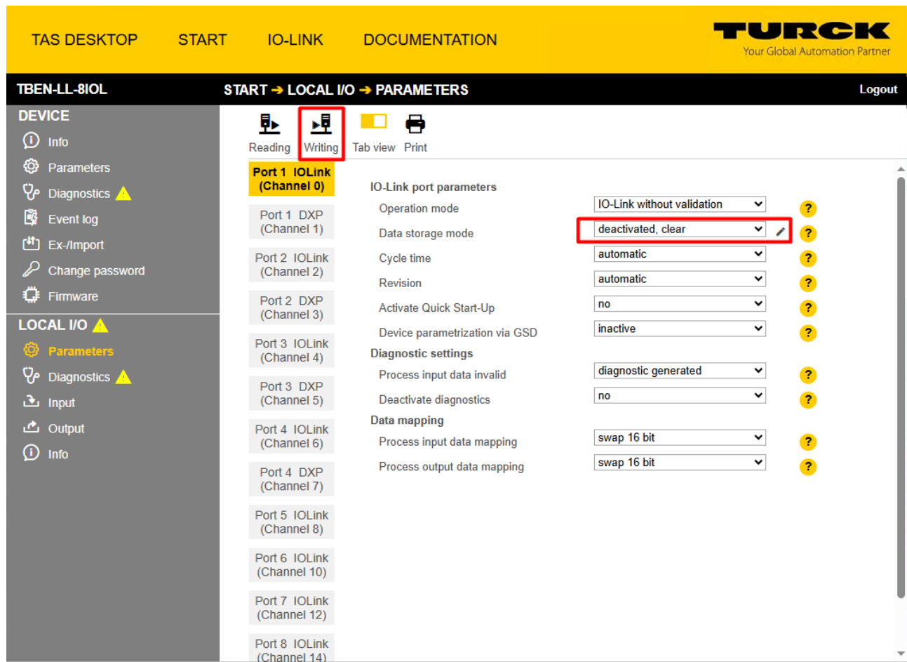
Fig. 100: TAS: deleting the data storage memory via parameters
